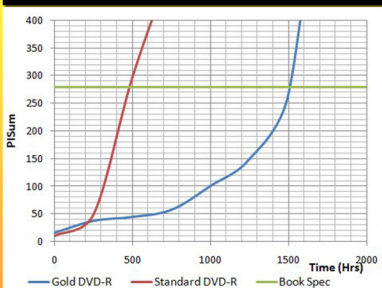
Aging Test: Gold Archival DVD-R vs Std DVD-R at 80C / 80% RH
